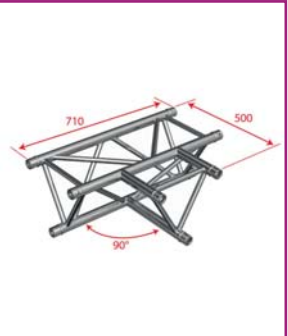
BT-TRUSS TRIO 29 - A017 Horizontal tee - 290 mm 90° - 3 directions Code : B03617
