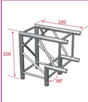
BT-TRUSS QUAT 29 - A003 Quatro angle - 90° - 2 directions
