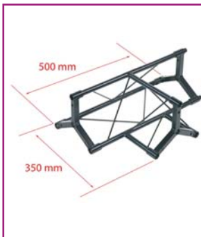
AG20-035 Horizontal tee - 200 mm - 3 directions
