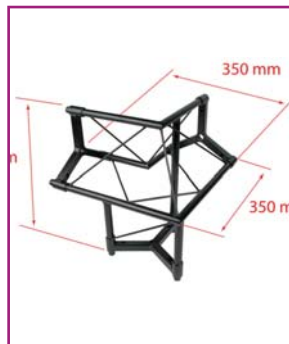
AG20-033 Angle - 200 mm 90° - 3 directions - Lower upright vertex
