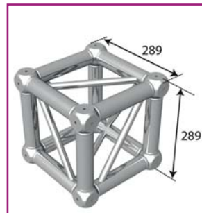
AGCUB290 Connection cube for 290 mm square truss
