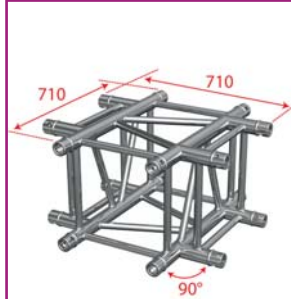
BT-TRUSS QUAT 29 - A016 Quatro angle - 90° - 4 directions
