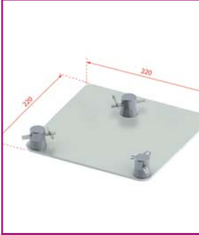
DECO22T-EM-B1 Trio 220 baseplate with conical couplers, spigot pins and Safety R-springs
