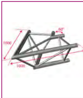
AG29-020 Angle 290 mm 2 directions 60°
