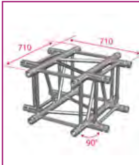
BT-TRUSS QUAT 29 - A016 Angle Quatro 4 directions 90°
