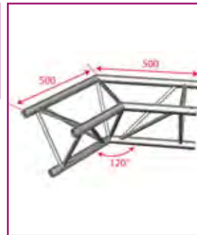
AG29-022 Angle 290 mm 2 directions 120°
